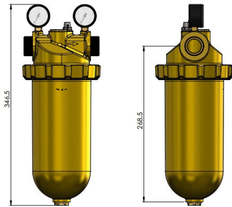
Filter 1" DN25
