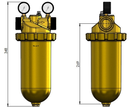
Filter 1 1/4" DN32
